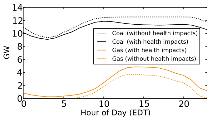
Fig. 4. July 2007 average dispatched load by hour of the day for coal and natural gas plants. The scenario including health impacts is shown by solid lines, and the scenario excluding health impacts is shown by dashed lines.
